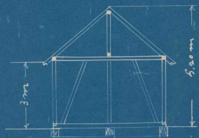
TVER-SNIT
